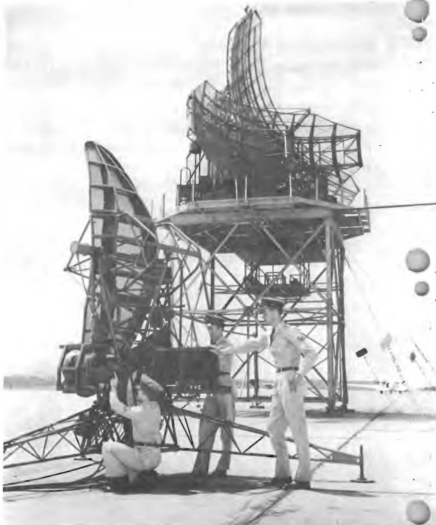
GCI - AN/TPS-10D Height Finder radar in foreground. AN/CPS-6 V beam search and height finder radar in background.
